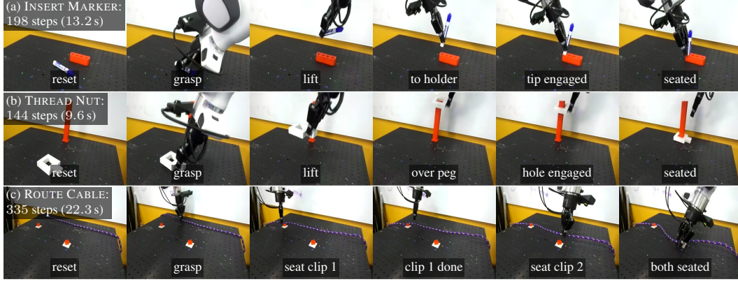
Figure 3: The three real-world tasks. Each row is the median-length successful held-out episode of the final-round HiL-IDQL+ Mulligan policy from the side camera, with frames at the rungs of each task’s stage ladder (Sec. C.3), not at even intervals. The median round-0 demonstration takes 12.7, 10.1, and 18.6 s. In (b), the policy carries the nut above the camera’s field of view between frames.
