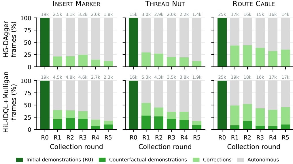
Figure 21: Composition of each round’s training data for the uniform-sampling (top) and Mulligan (bottom) collection campaigns, as a share of valid frames. The number above each bar is the round’s count of human-controlled frames. Both campaigns collect the same number of episodes per round. The uniform-sampling campaign’s data train HG-Dagger, and the Mulligan campaign’s data train both HG-Dagger+ Mulligan and HiL-IDQL+ Mulligan .
