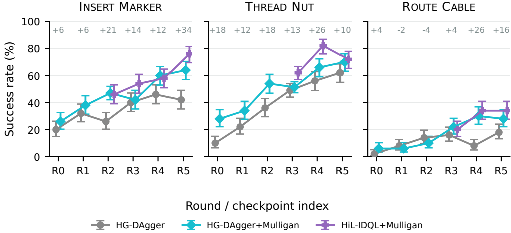
Figure 10: Per-arm full-success results for the policies in Fig. 5, with HG-Dagger (grey), HG-Dagger+Mulligan (teal), and HiL-IDQL+Mulligan with critic reranking (purple) as separate series. The top row gives the per-round delta of the policy deployed in the Mulligan campaign over the uniform-sampling HG-Dagger baseline in percentage points. Intervals are Wilson-score one-standard-error ( z=1 ). The ROUTE CABLE panel shows full-episode success for rounds R0–R5, scored on one shared block of 50 initial states.
