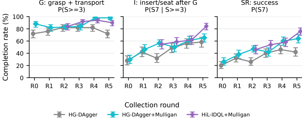
Figure 17: Per-stage decomposition on INSERT MARKER across rounds: grasp+transport (left), insertion/seat conditioned on grasp (middle), and overall success (right), with Wilson-score one-standard-error intervals ( z=1 ). The collection arm retains a grasp-stage advantage at R5, while reranking improves conditional insertion success. R5 uses the stage labels of the headline three-arm session.
