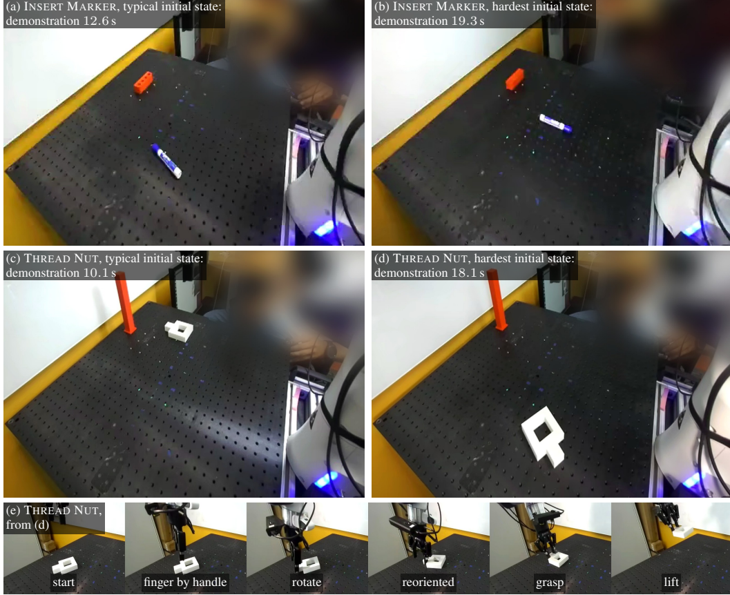
Figure 22: Typical and hardest initial states of INSERT MARKER and THREAD NUT in round-0 teleoperation. (a)–(d) are the first frames from the side camera next to the robot base, which is on the right (operator blurred). Each hardest initial state is the first state of the task’s longest round-0 demonstration, with the object near the minimum of its x range and pointing toward the robot. Each typical initial state comes from a median-length demonstration whose object points away from the robot. The typical INSERT MARKER initial state lies at nearly the same x as the hardest one. (e) From the hardest THREAD NUT initial state, the robot places a finger next to the handle with the gripper yawed 180^\circ from the grasp orientation, rotates the nut, and then grasps it, seen from the opposite side camera. The three longest round-0 demonstrations of each task all start with the object within 21^\circ of pointing toward the robot.
