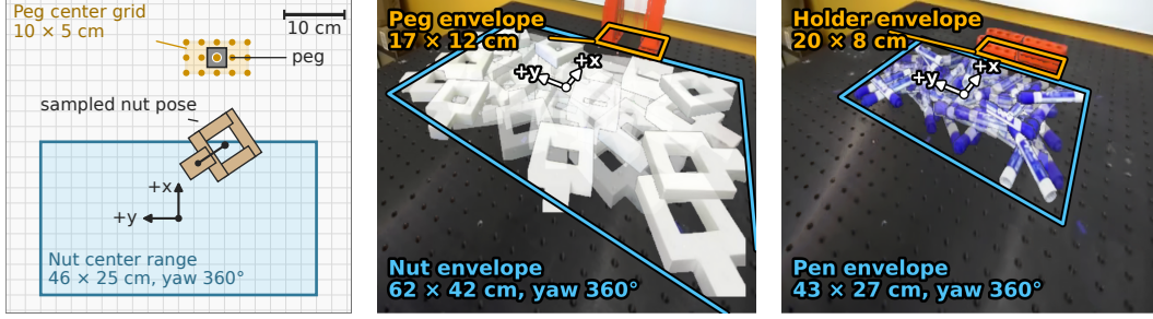
Figure 4: Left: the THREAD NUT reset-helper card from which the operator places each episode’s objects. The nut center is sampled uniformly over the blue range at any yaw, and the peg is snapped to the orange grid (all three tasks in Sec. E.4). Middle and right: side-camera overlays of boundary and interior reset poses for THREAD NUT and INSERT MARKER, with each object’s envelope, its center range grown by its reach, outlined and labeled. The ROUTE CABLE overlay is in Fig. 1, left.
