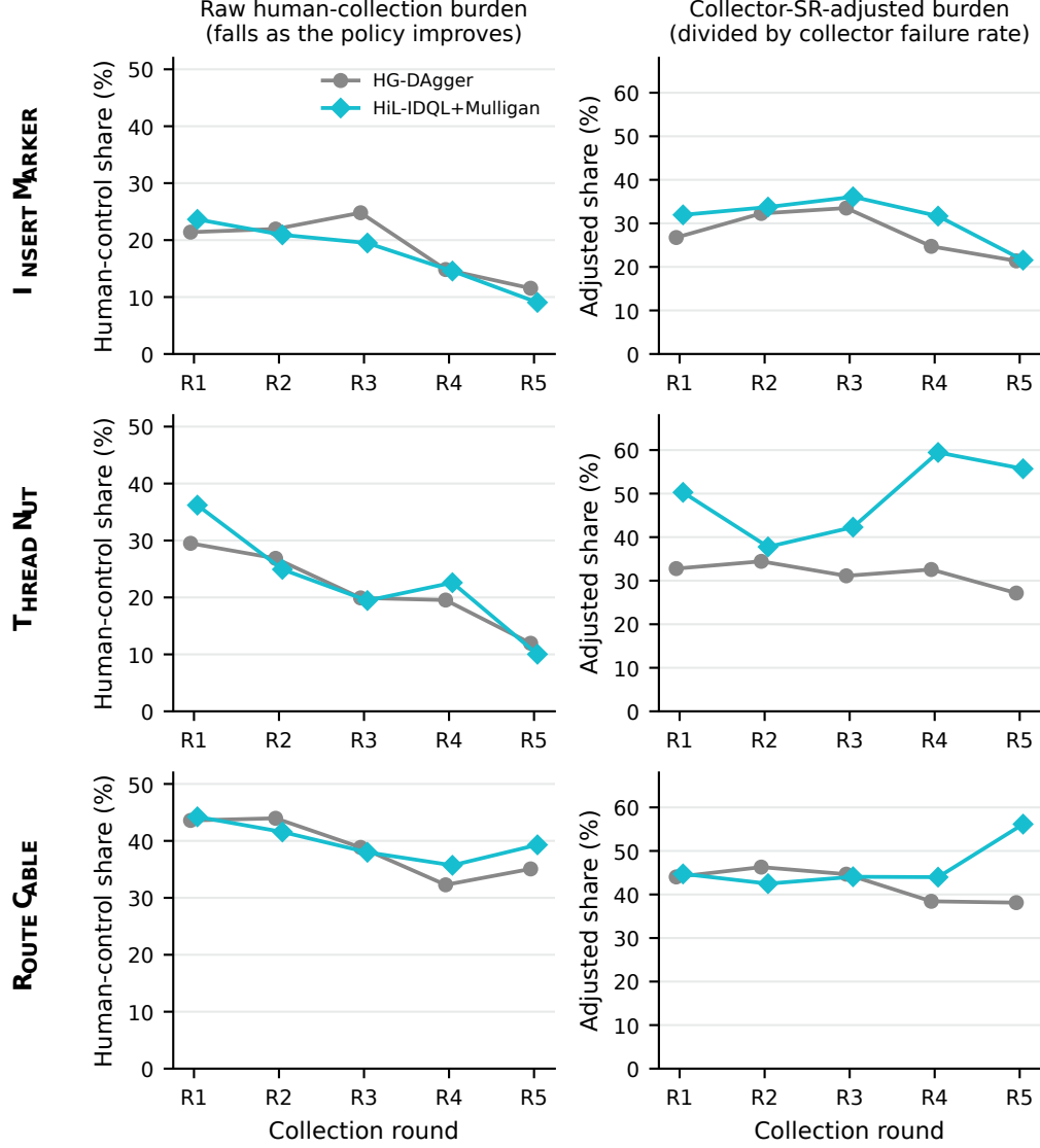
Figure 20: Human collection burden over DAGger rounds on INSERT MARKER (top), THREAD NUT (middle), and ROUTE CABLE (bottom, 100-episode increments, each normalized by the fresh-episode-weighted held-out success of the policies that collected its source rounds), for the uniform-sampling (grey, HG-DAGger) and Mulligan (teal, HiL-IDQL+ Mulligan ) collection campaigns. Left: raw burden (share of frames under human control in fresh collection episodes). Right: the same share normalized by the collection policy’s failure rate ( 1 - \text{SR} ). On ROUTE CABLE, where complete success is still near the floor, the normalization is close to the identity.
