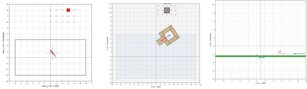
Figure 25: Per-episode reset-helper schematics for placing objects at each sampled initial state. Each card shows the allowed object-center grid, the chosen locations, and the sampled object poses (position and yaw) in table coordinates. Left: INSERT MARKER (pen + holder). Middle: THREAD NUT (nut + peg). Right: ROUTE CABLE (cable + two clips).
