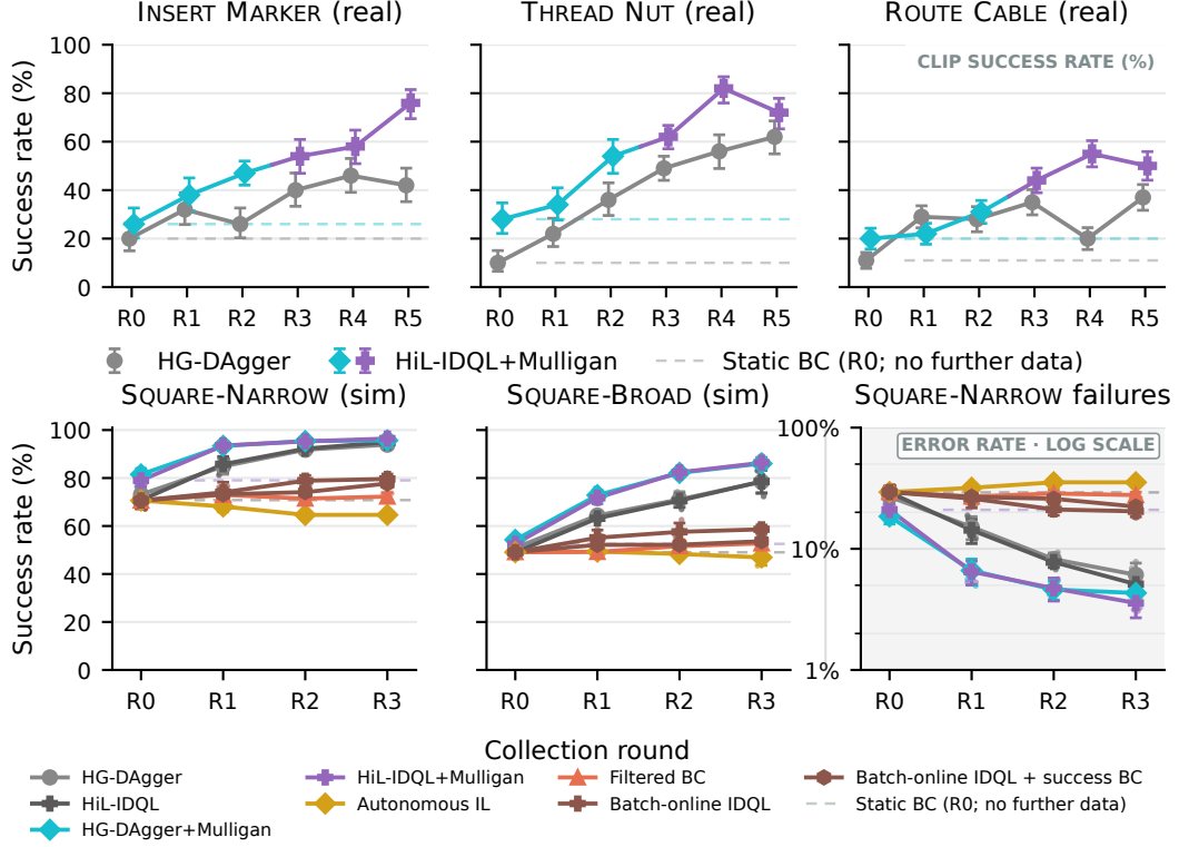
Figure 5: Held-out performance over Dagger rounds, real world (top) and simulation (bottom). Real-world panels show full-task success on INSERT MARKER and THREAD NUT and clip success rate on ROUTE CABLE, the fraction of two clips seated (per-method full-task success in Sec. B.1). Real-world whiskers are \pm 1 SE over 50 episodes, or 100 for the pooled INSERT MARKER R2 HiL-IDQL+Mulligan point and both THREAD NUT R3 points (Sec. D). SQUARE-NARROW failures ( 100 - \text{SR} ) use a log scale. Dashed lines mark each campaign’s static round-0 policy. For real-world HiL-IDQL+Mulligan, teal points use the actor alone and purple points add critic reranking.
