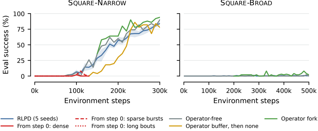
Figure 29: HiL-SERL eval success per session (one seed each) against RLPD (five-seed mean, shaded \pm standard error) on SQUARE-NARROW (left) and SQUARE-BROAD (right). Operator forks branch from the operator-free run at 150k and 200k. The operator-buffer arm continues the sparse-burst session from 130k with no operator.
