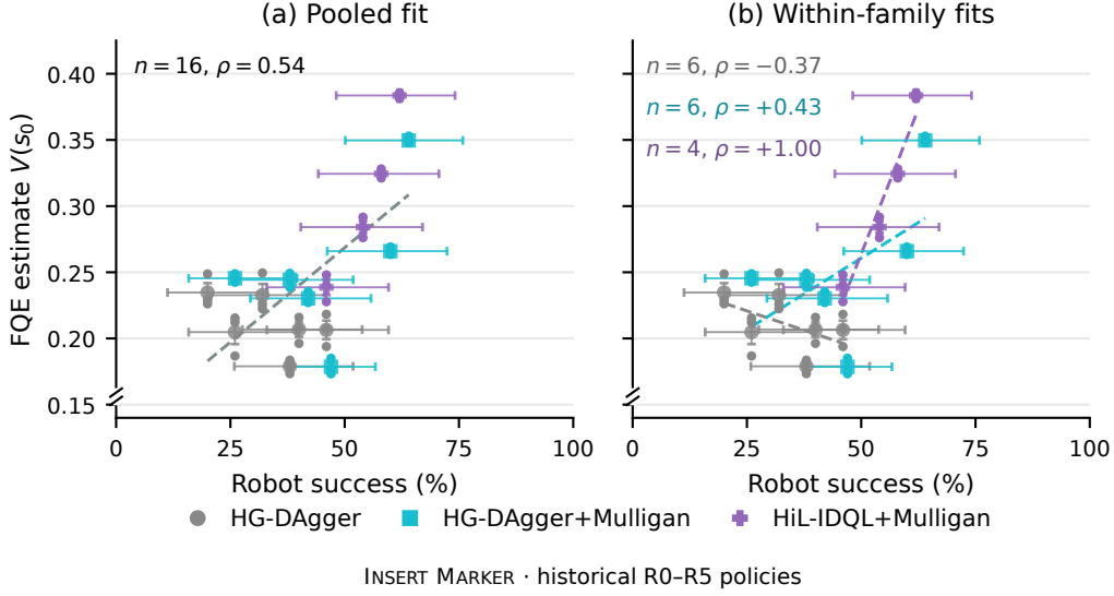
Figure 31: FQE backtest on 16 historical INSERT MARKER policies, shown with (a) a pooled fit and (b) separate fits by policy family. Dashed lines are descriptive least-squares fits, and \rho denotes Spearman correlation. The value axes are zoomed to [0.14, 0.425] . Markers average three evaluator seeds, small dots show individual seeds, and vertical whiskers give one standard error across seeds. Horizontal whiskers are Wilson 95% intervals from recorded robot counts (50 attempts per policy, except 100 for round-2 DP), without adjustment for repeated initial states. Evaluators use \gamma = 0.995 , timeout bootstrapping, and their final 40k checkpoint. FQE scores every policy on the same 150 round-5 reset images (50 initial states), but each robot success rate comes from that policy’s own historical round. The round-5 BoN point uses the original 31/50 critic, not the critic selected later. Because the policies are related and the two axes use different initial-state distributions, the pooled fit is hard to interpret.
