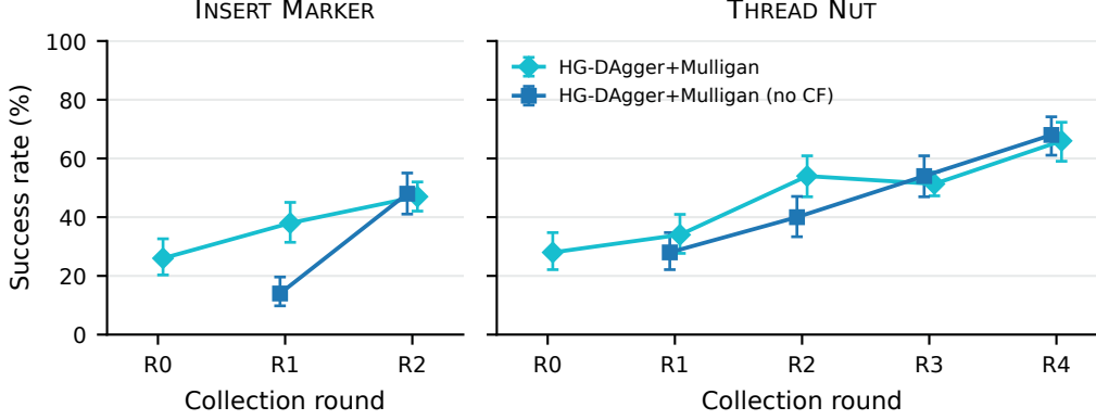
Figure 15: Counterfactual-demonstration ablation on INSERT MARKER (left) and THREAD NUT (right): held-out success rate over DAgger rounds for HG-Dagger+Mulligan with and without CF demos, with Wilson-score one-standard-error intervals ( z=1 ). Each panel ends at the last round with a no-CF evaluation (INSERT MARKER R2, THREAD NUT R4). R0 is the shared source actor, shown once. Most points use 50 episodes, and the with-CF INSERT MARKER R2 and THREAD NUT R3 points pool 100 and 150 episodes. Removing counterfactuals lowers early-round success more on INSERT MARKER than on THREAD NUT, and on both tasks the arms converge as corrections accumulate.
